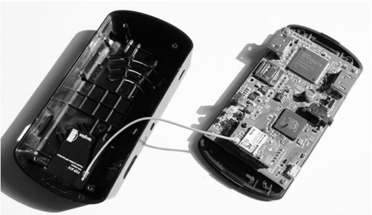
A NeTV sporting the Chumby logo
