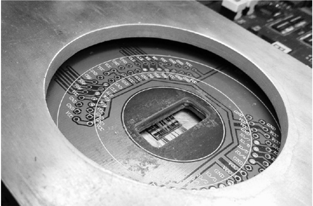
The probe card, up close
