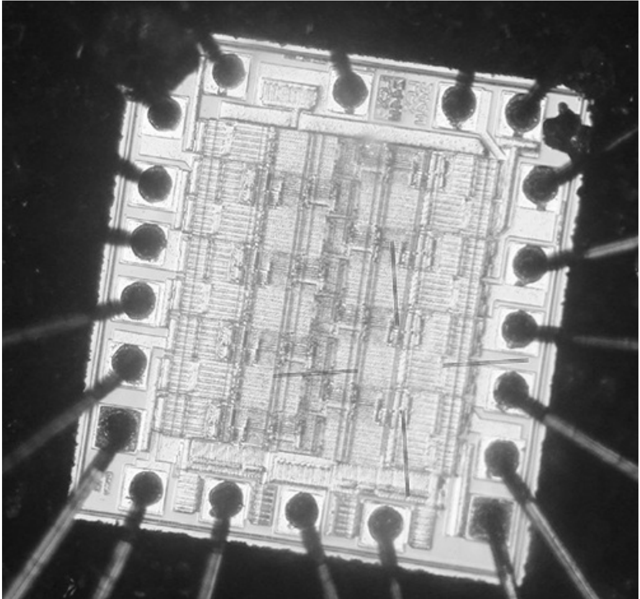
The silicon inside the fake ST19CF68
