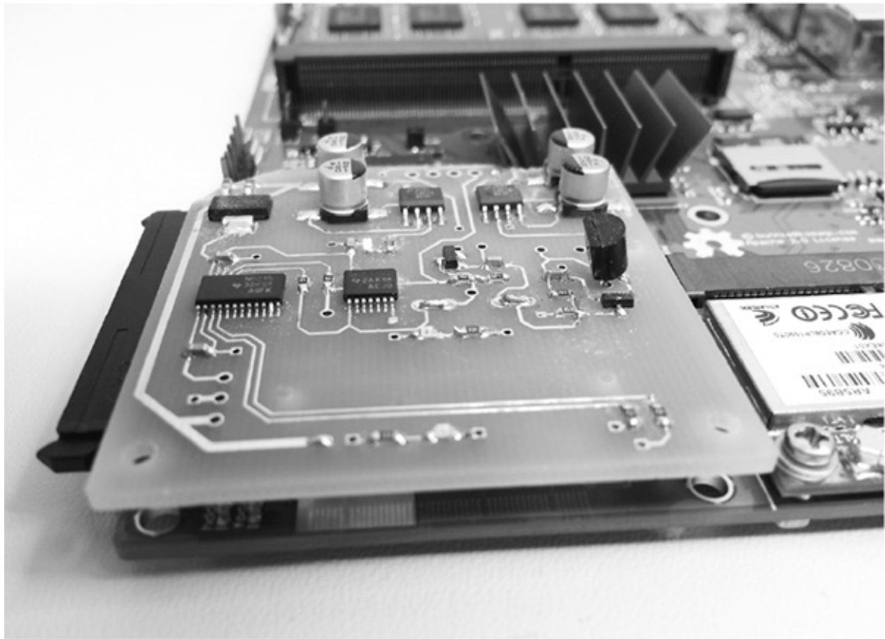
A prototype CrypTech expansion board, plugged into the
