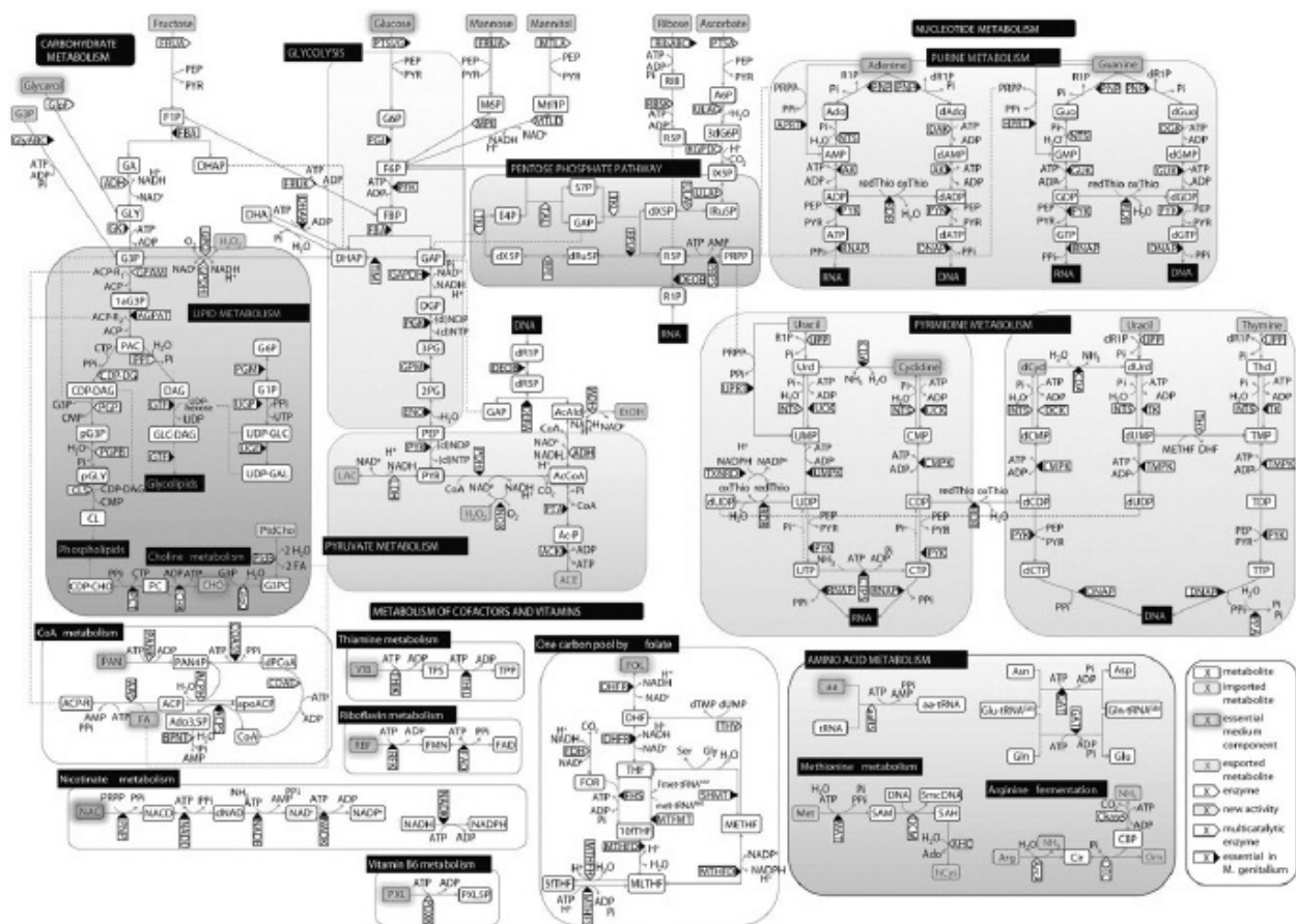
Mycoplasma pneumoniae's metabolic pathway
