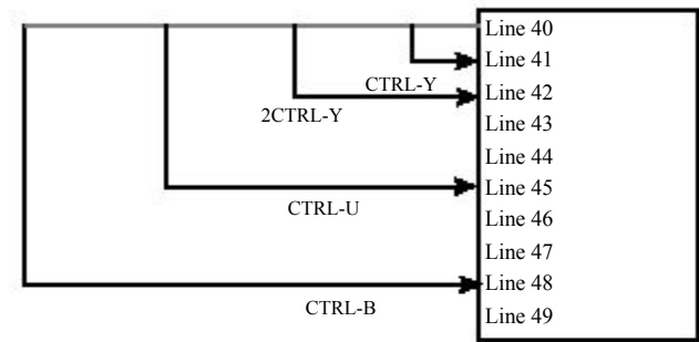
Figure 18.10 Scrolling commands.
