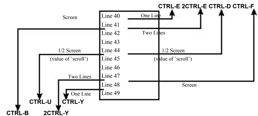
Figure 18.11 More scrolling commands.
