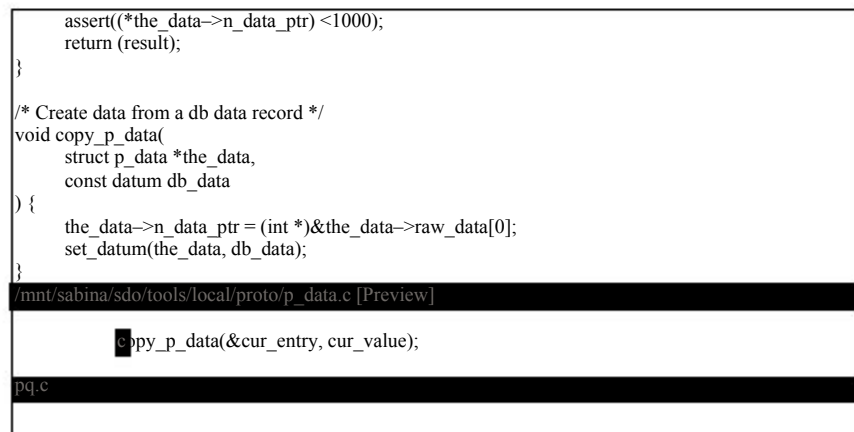
Figure 23.11 :ptag example.
