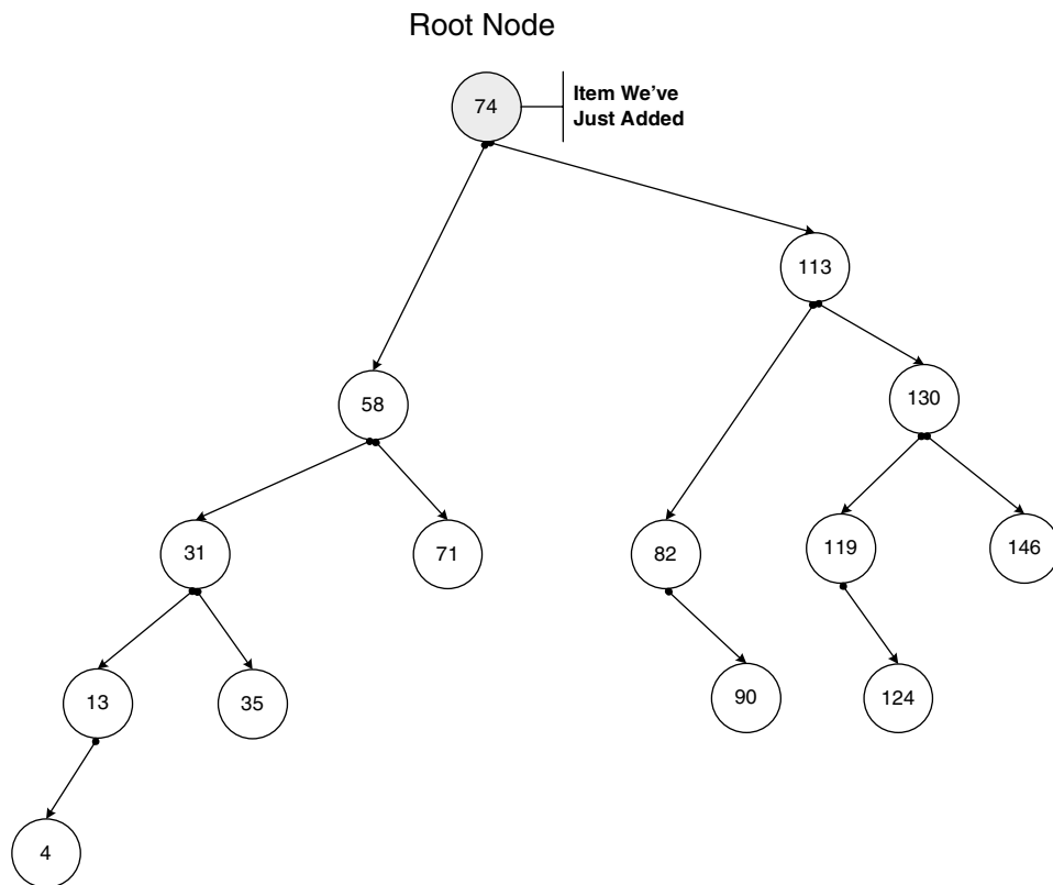
Figure 5.5 Binary after splaying process. The new item is now the root node, and the rest of the tree is centered on it.
