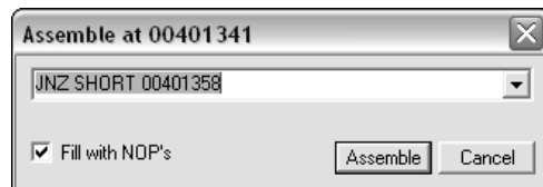
Figure 11.7 The Assemble dialog in OllyDbg .
