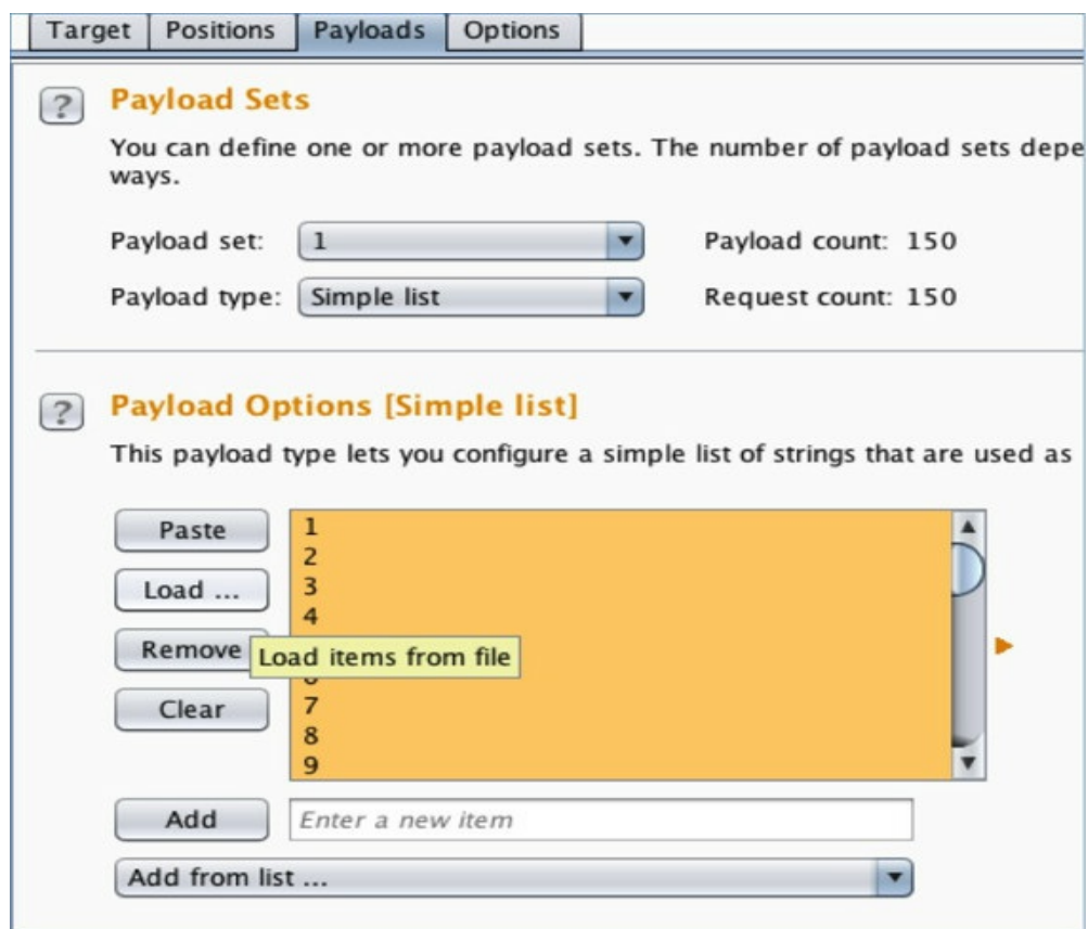
Burp List
