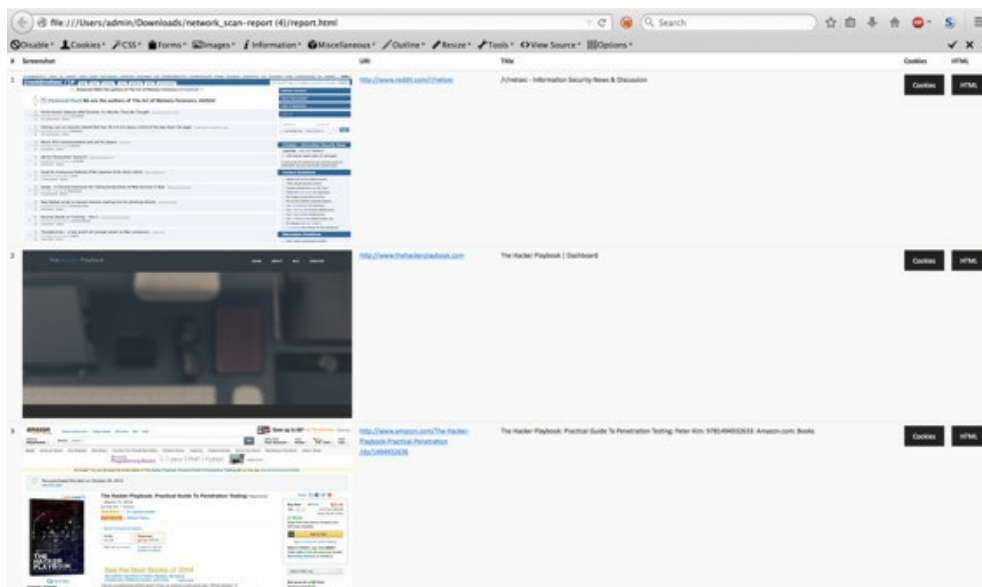
WAMP Results
