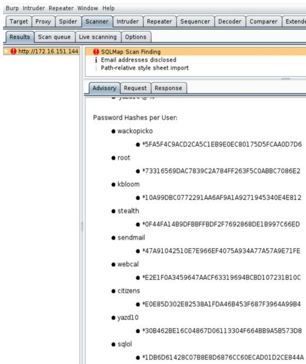
SQLMap Results
