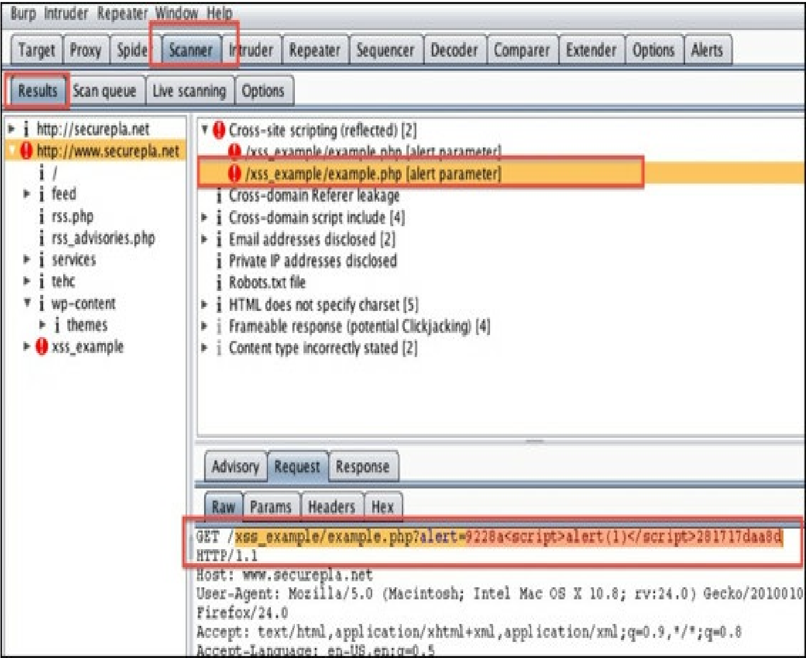
Scan Results
