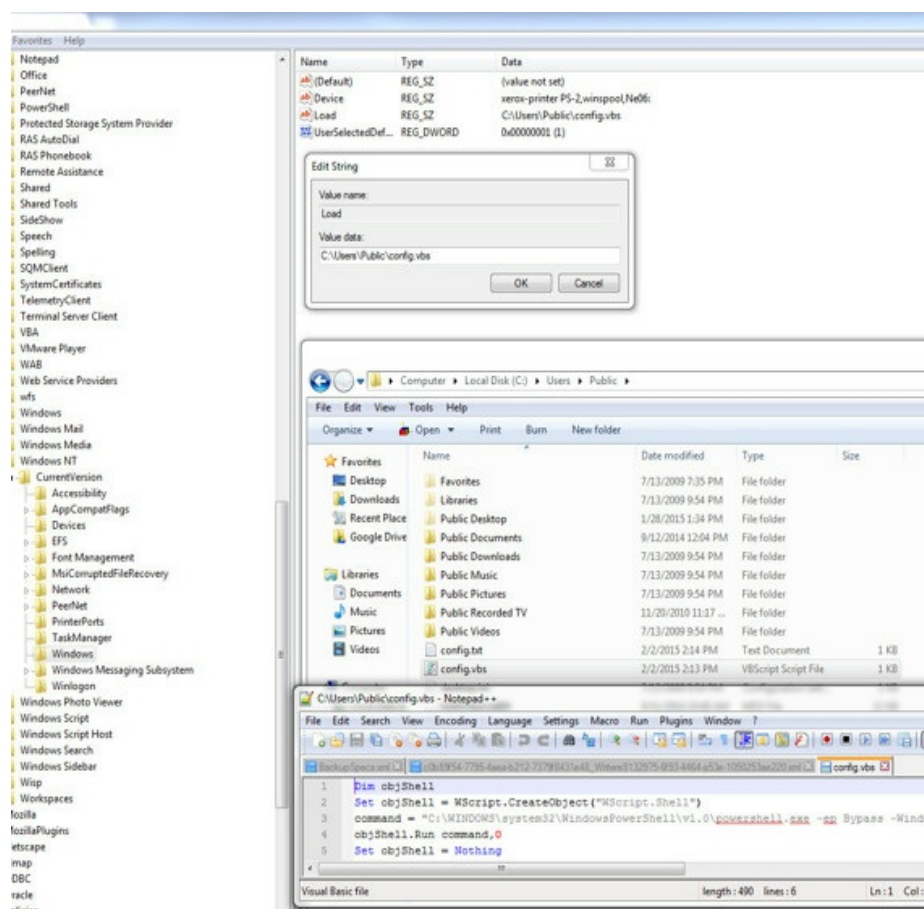
Registry Persistence
