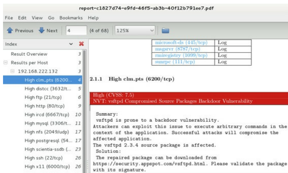
OpenVAS – Findings
