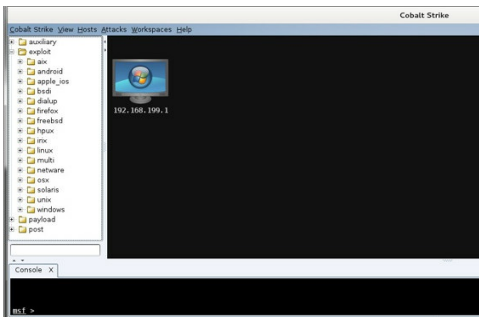
Cobalt Strike
