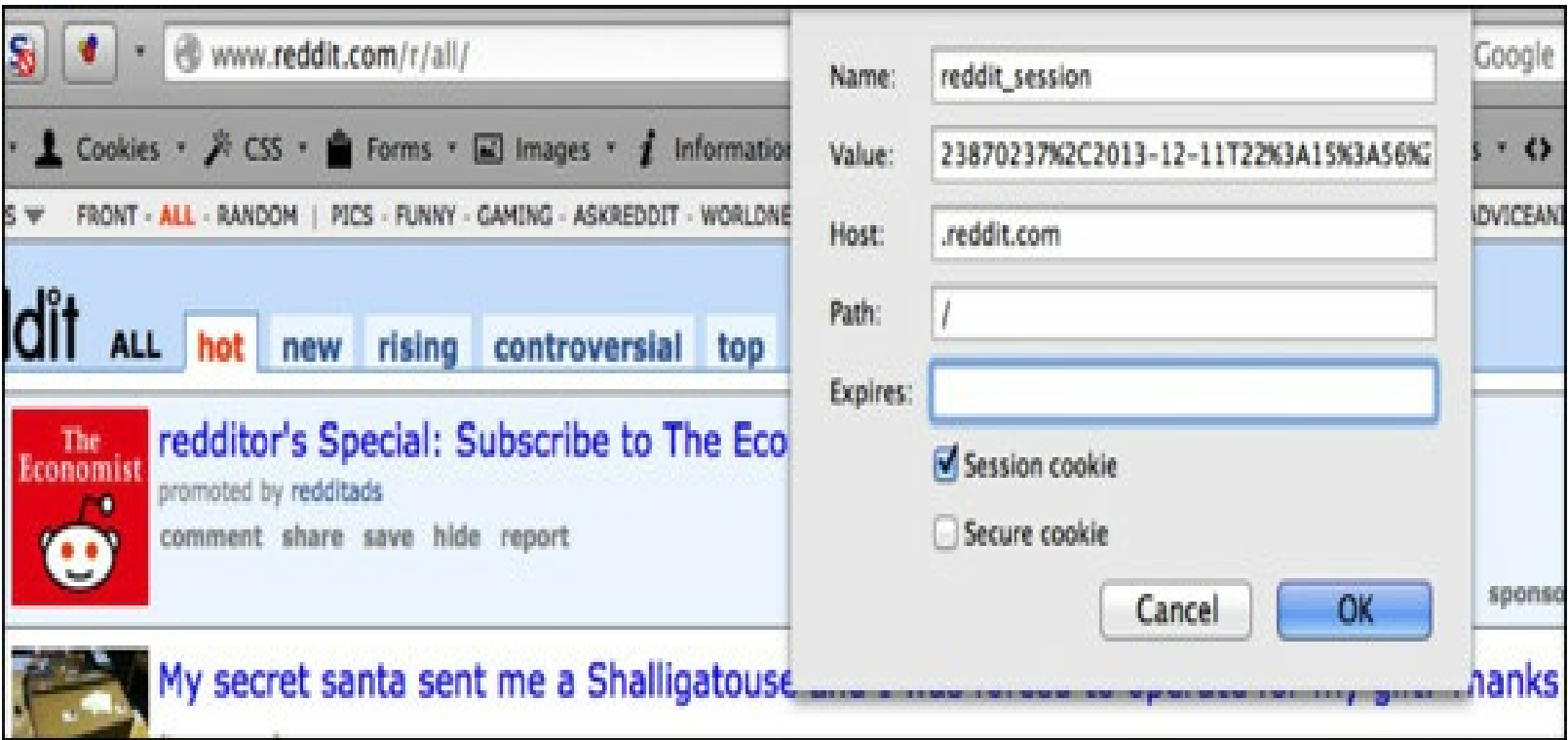
Replacing Cookies
