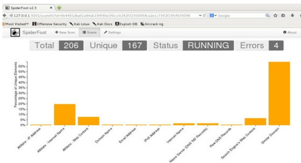
SpiderFoot Report
