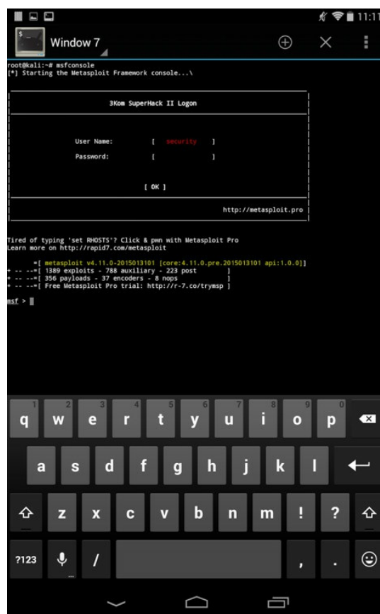
Nethunter - Metasploit
