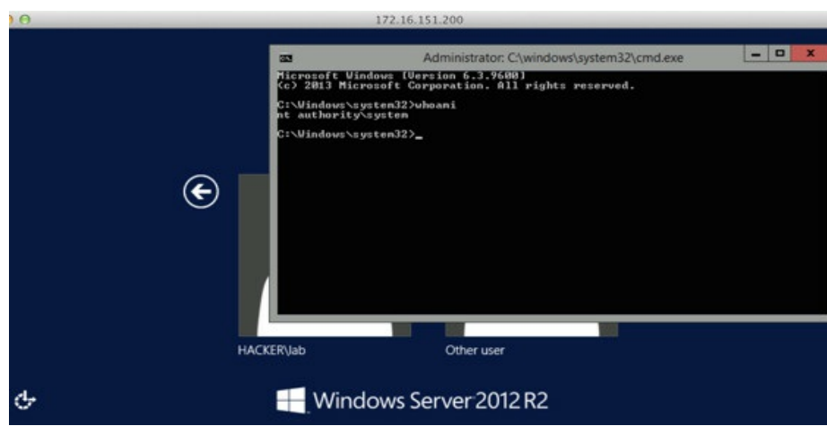
Sticky Key
