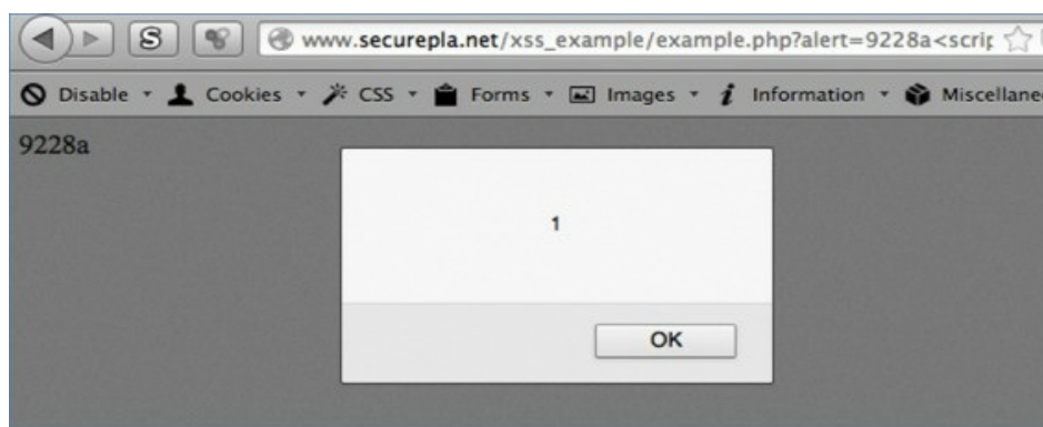
XSS Example
