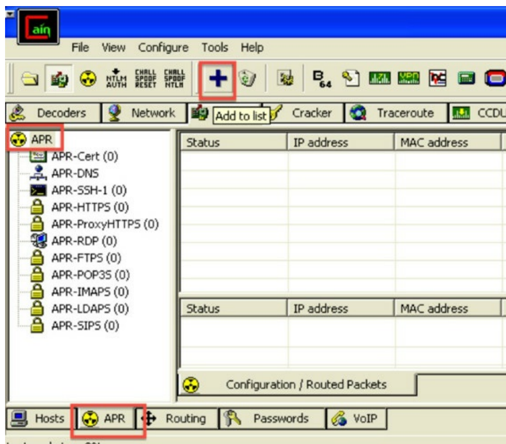
APR List
