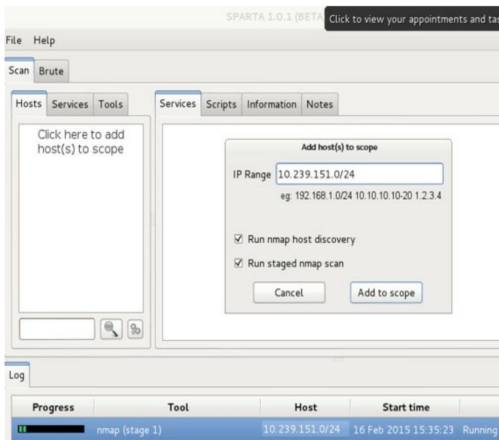
SPARTA – Scan
