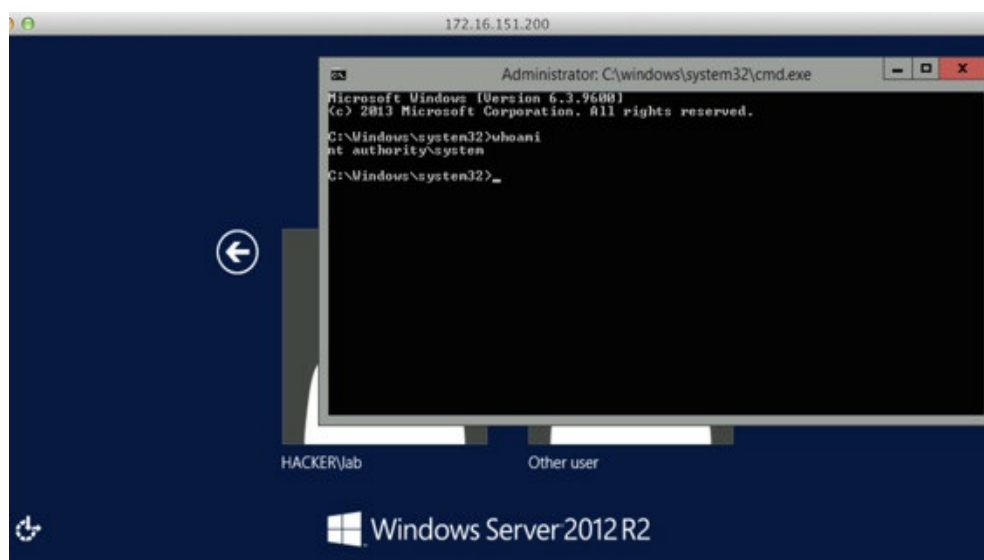
Sticky Keys
