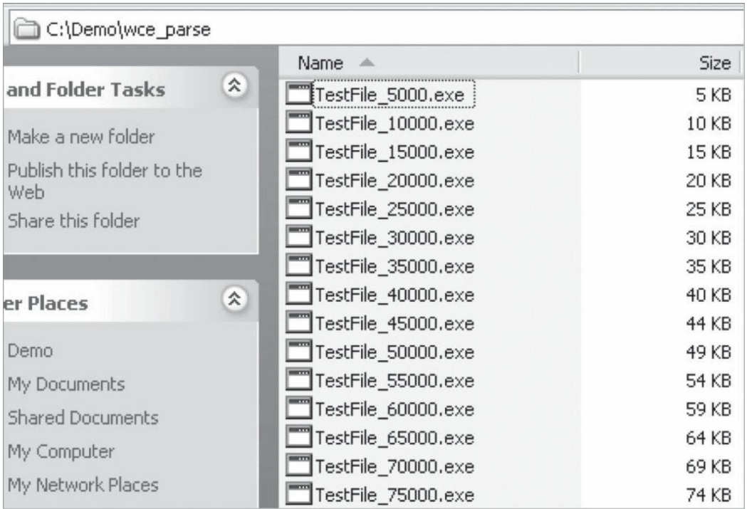
Figure 126 - Evade Output
