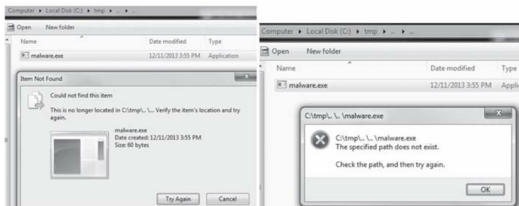
Figure 148 - Hiding Files
