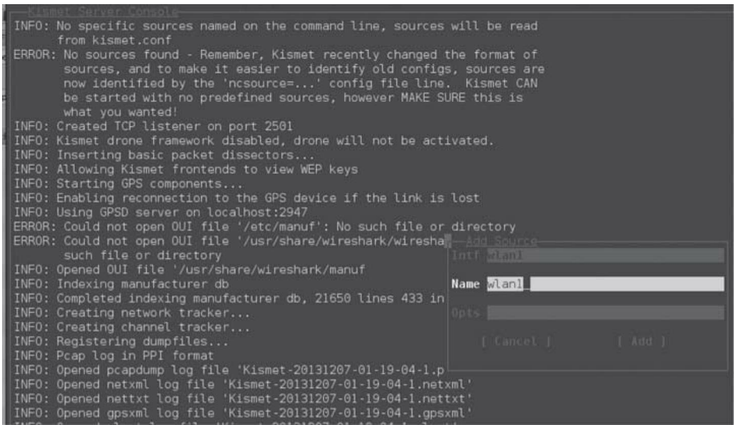
Figure 115 - Kismet Configuration
