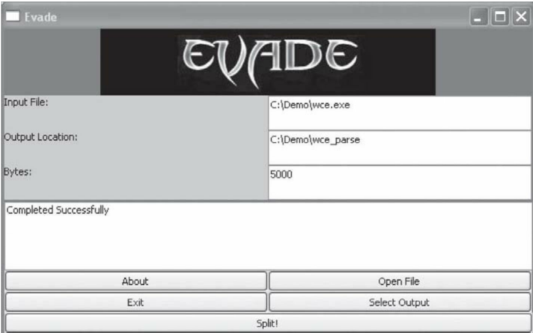
Figure 125 - Evade
